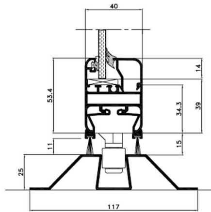
Low Sill
