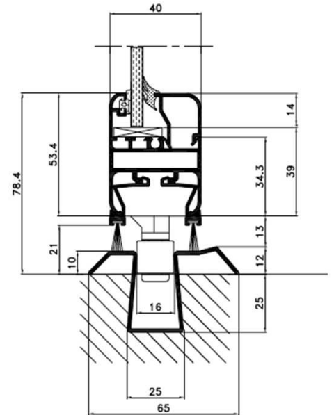
Flush Sill
